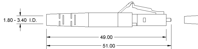
LC Impact Mount® Connector
